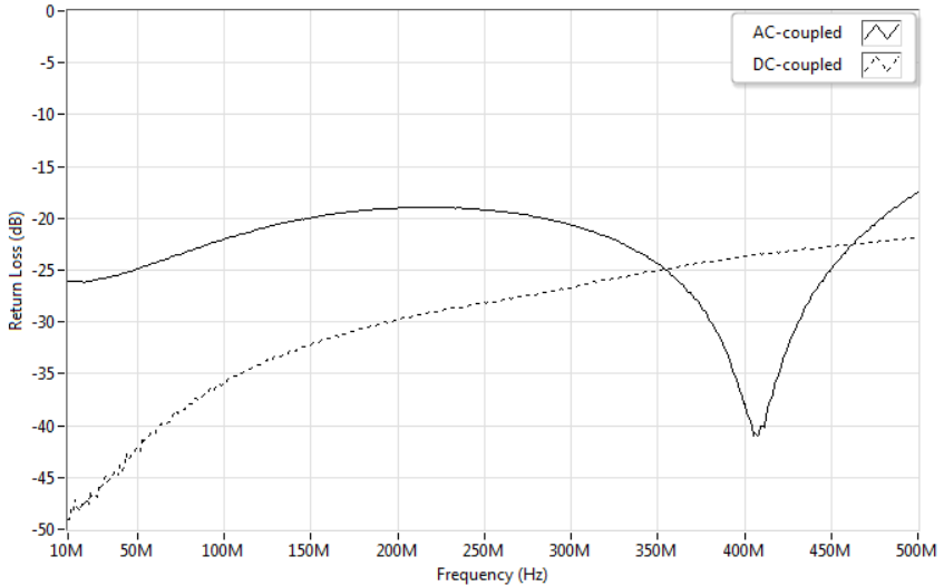
Figure 11. Input Return Loss, Measured
