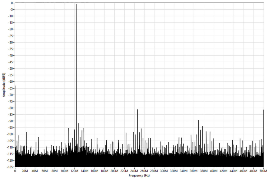
Figure 5. DC-Coupled Single Tone Spectrum (123.1 MHz, -1 dBFS, 1 kHz RBW), Measured
