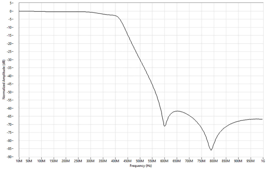
Figure 10. DC-Coupled Frequency Response Zoomed In, Measured
