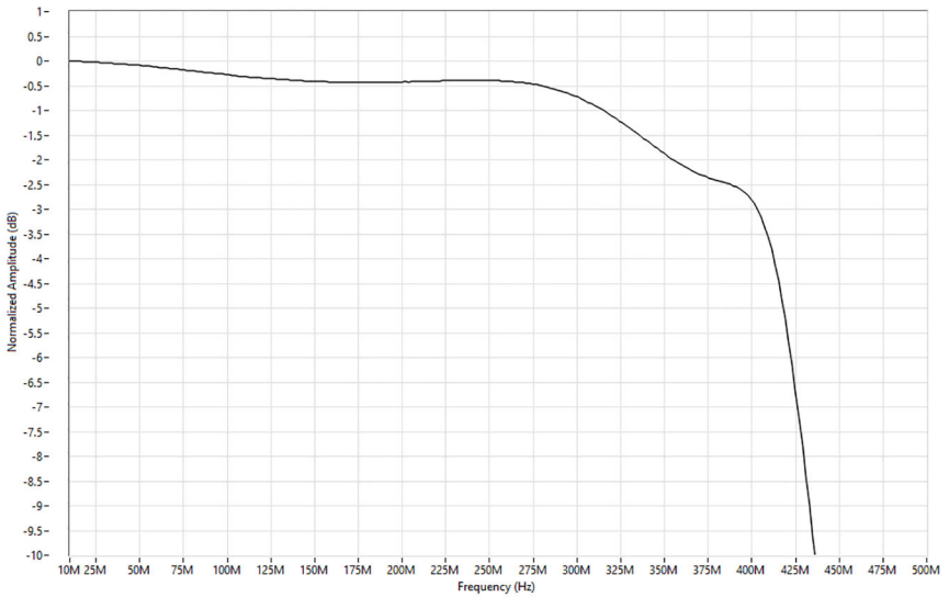
Figure 10. DC-Coupled Frequency Response Zoomed In, Measured
