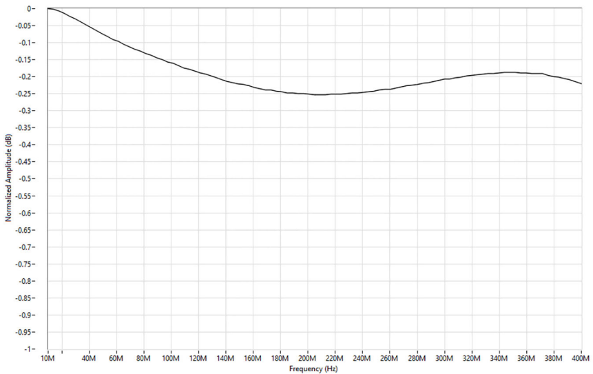
Figure 8. AC-Coupled Passband Flatness for Full Scale Input Supported Frequency Range, Measured
